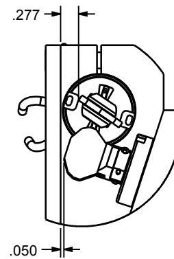
DIMENSIONS FROM THE F-THETA LENS CUTOUT TO MIRRORS IN EXTREME POSITIONS
